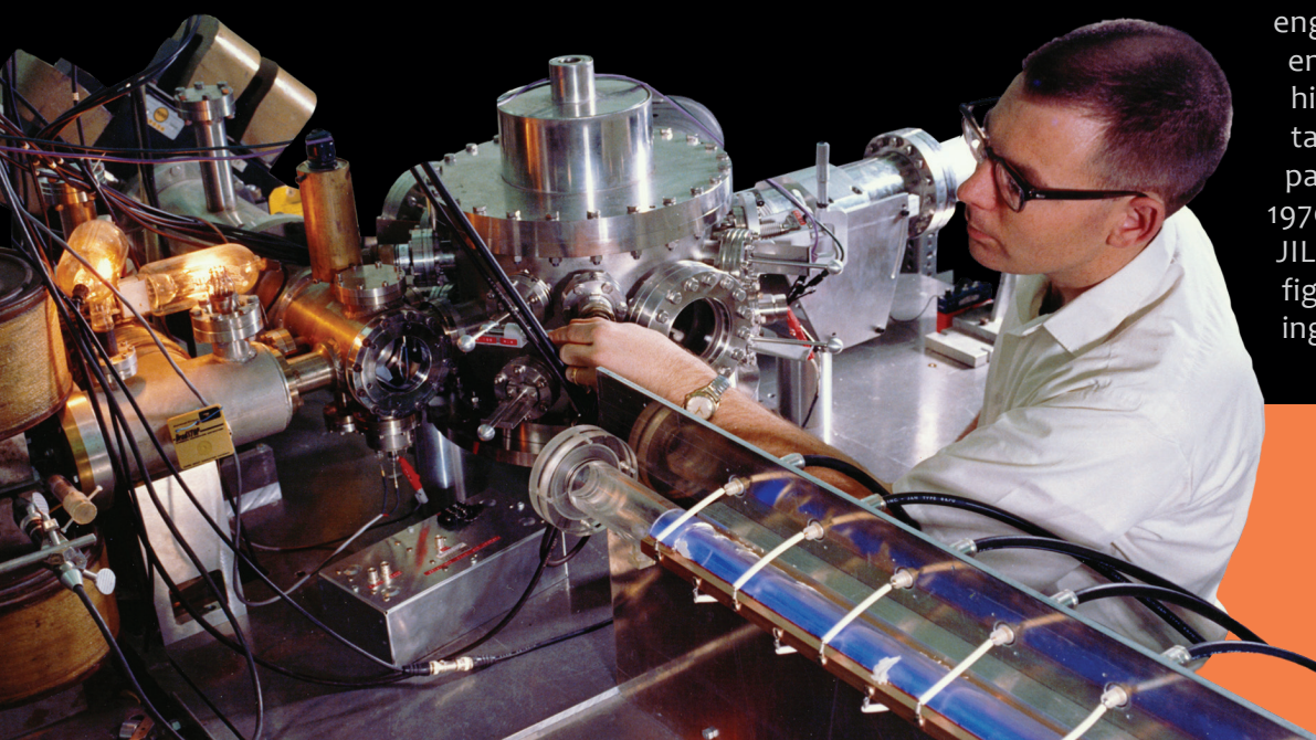
The negative photo ion detachment apparatus first pioneered by physicists and JILA founders Lewis Branscomb and Steve Smith. Later W. Carl Lineberger modified the apparatus for his own experiments using a tunable dye laser. Credit: JILA
