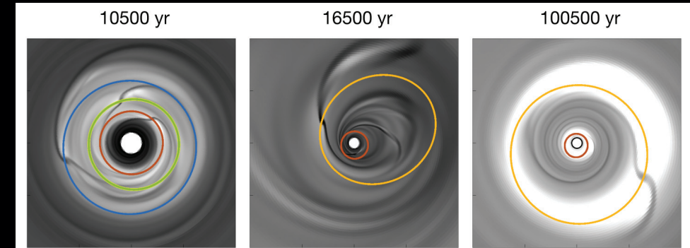
Computer simulation of the evolution of a planetary system and its gas disk. Credit: Nick Moekel, Institute of Astronomy, University of Cambridge, UK
