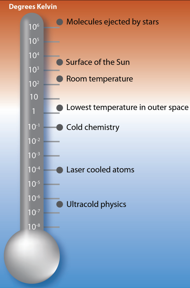
Temperatures throughout the Universe. Credit: Kristin Conrad, JILA
