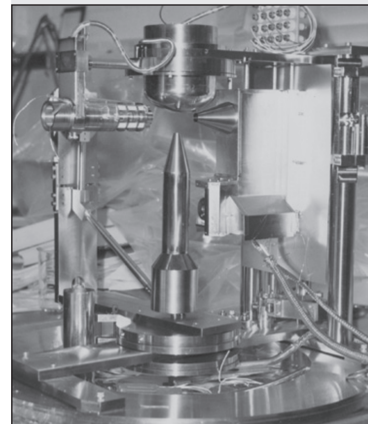
Electron impact ionization apparatus. A gas jet directed downward from the dome in the center crosses an electron beam from the electron gun at the left. Scattered incident electrons and electrons knocked-out of the target atoms are detected by the electron analyzer at the right and by the moveable analyzer that is positioned below the scattering center. Credit: JILA
