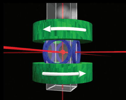
JILA BEC trapping and cooling apparatus. Credit: The Wieman group
