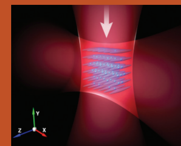
Artist's conception of a 2D clock lattice. Credit: The Ye group and Greg Kuebler, JILA
