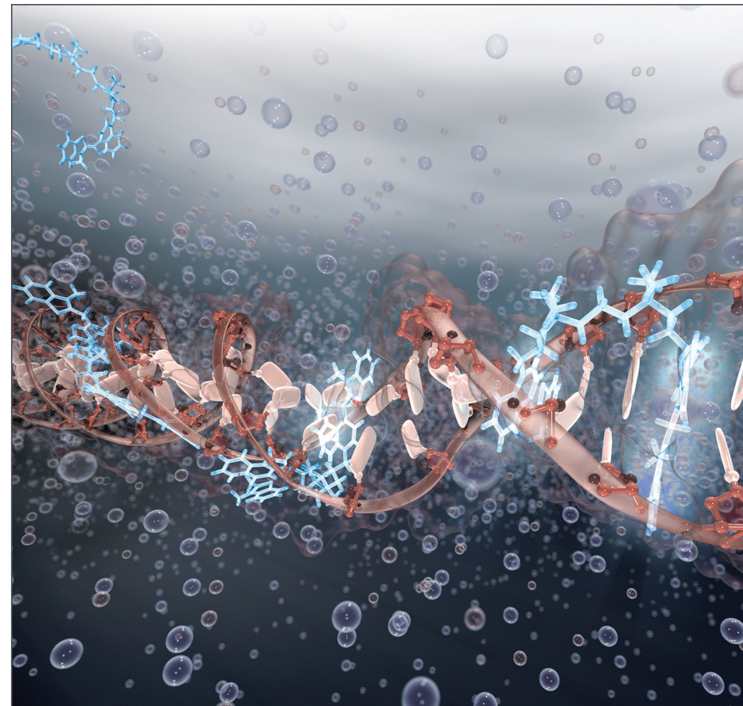
Four modes of interaction of a drug molecule (blue) with a strand of DNA.
